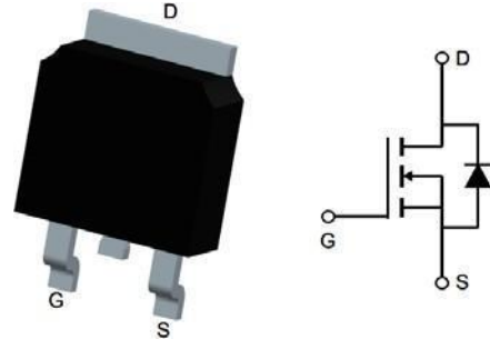
TO-252
